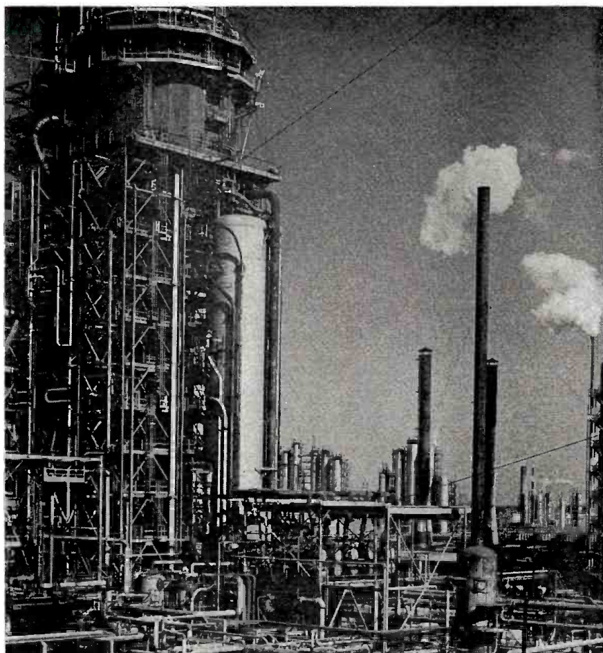
A panoramic view of the Baytown maze of Cat Cracker #2 in the immediate foreground.
